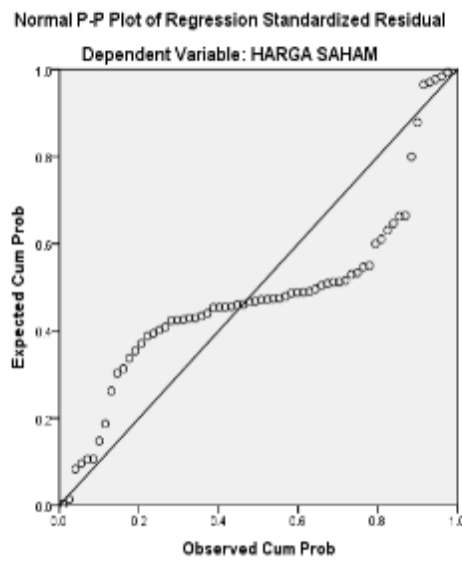
Figure 2. Plot Graph of Normality Test Before Transformation
