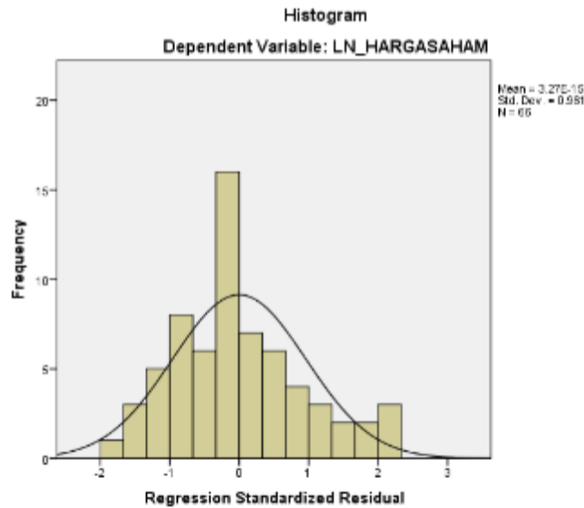
Figure 3. Histogram Graph Normality Test After Transformation
