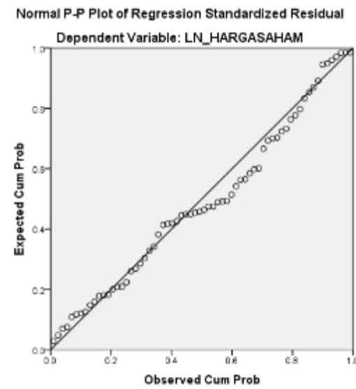
Figure 4. Plot Graph of Normality Test After Transformation
