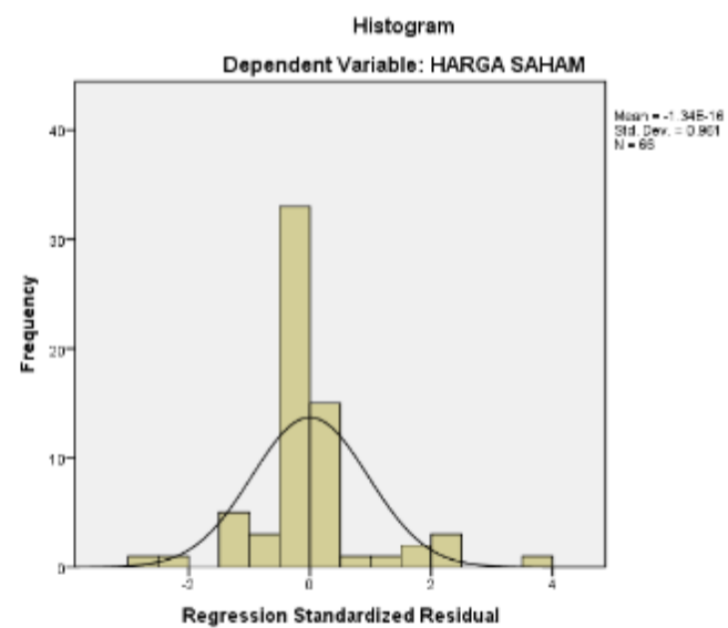
Figure 1. Histogram Graph Normality Test Before Transformation
